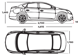
Car Dimensions
